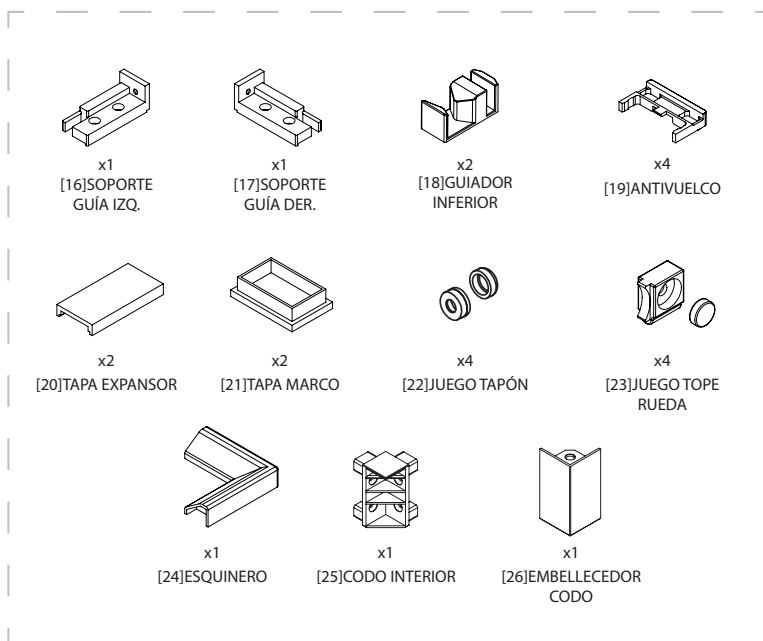
KIT ACC. ABS BRENTA KB7012
